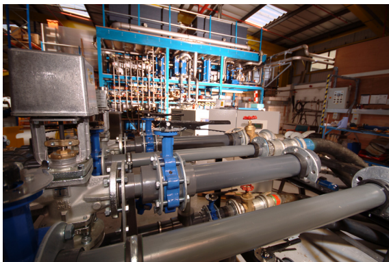
Tricool Thermal's test rig
